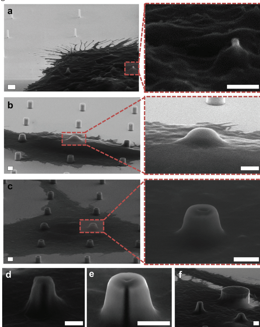
Figure 5. A variety of nanopillar-cell interactions , (a) fibroblasts fully spread on top of ~220 nm nanopillars, some nanopillars tips were visible in SEM images, suggesting full nanopillar penetration through the cell, (b) a fibroblast fully spread on 1 \mu m diameter solid nanopillars, where most pillars were buried under the cell body, (c) fibroblast spread on top of hollow shaped array of nanopillars, the membrane conformed to the shaped of these nanostructures and appears to adhere to the inside of the hollow nanopillars. (d)-(f) membrane conformed to the shape of x-shaped and c-shaped nanopillars forming contacts on the sidewall grooves. All scale bars represent 1 \mu m.
