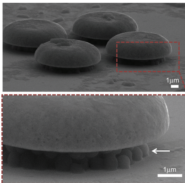
Figure 9. 70° tilted SEM micrograph revealing mushroom shaped structures with 5 \mu\text{m} diameter stems. Several S. aureus cells were clustered at the stem of these structures (arrow).
